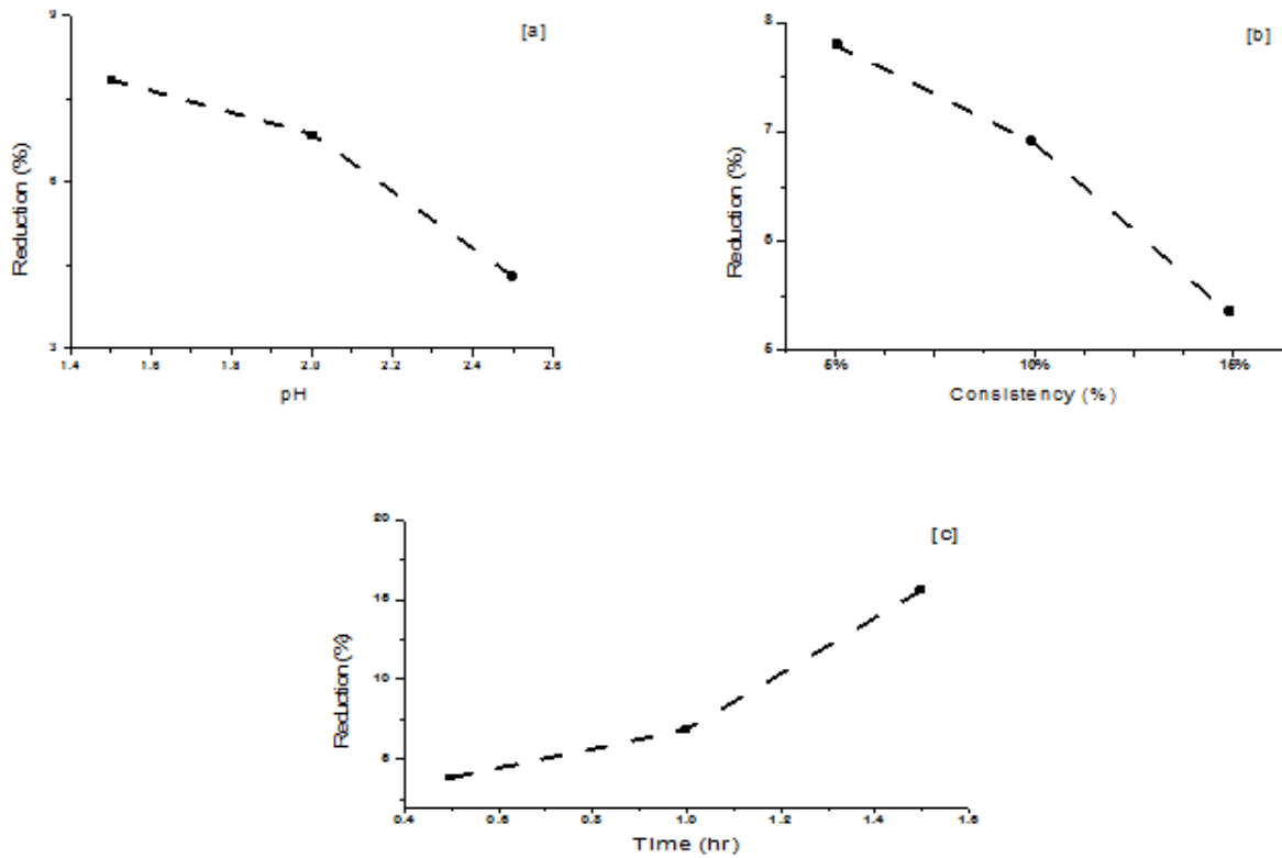
Fig. 2 Effects of [a] pH [b] consistency (%) and [c] time (hr) on the reduction in Holocellulose content due to acid pre-treatment
