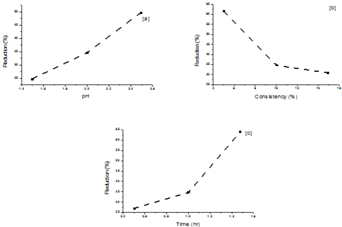
Fig. 3 Effects of [a] pH [b] consistency, % [c] time on the lignin content due to acid pre-treatment
