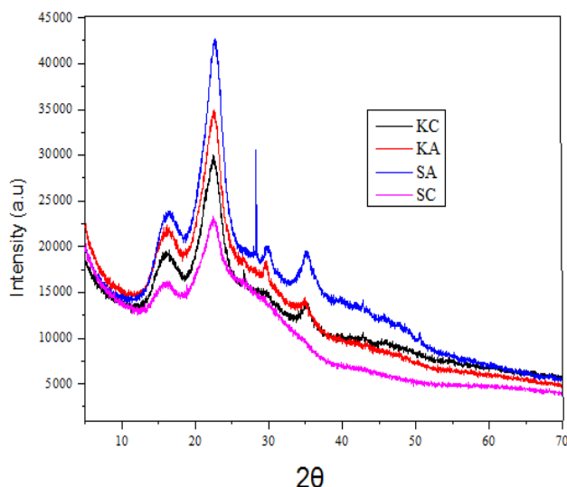
Fig. 10 X-ray diffraction pattern of kraft and soda pulp (Untreated and acid treated)
