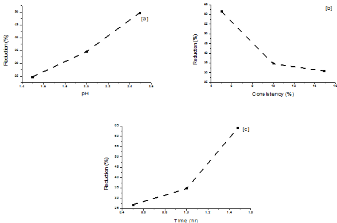
Fig. 4 Effects of [a] pH [b] consistency (%) and [c] time (hr) on the reduction in Extractives content due acid pre-treatment
