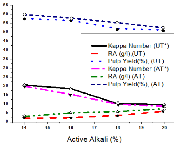
Fig. 7 Effects of acid pre-treatment on kraft pulping of wheat straw (*UT- Untreated, *AT- Acid treated)
