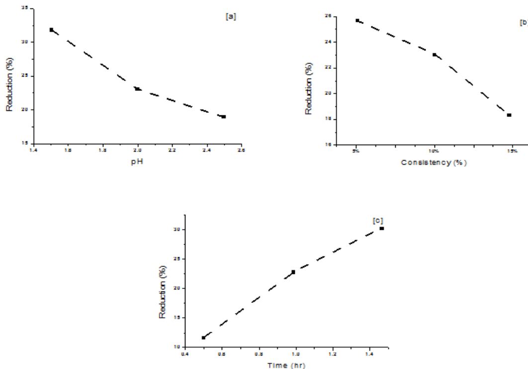
Fig.5 Effects of [a] pH [b] consistency, % [c] time (hr) on reduction in Silica content due to acid pre-treatment
