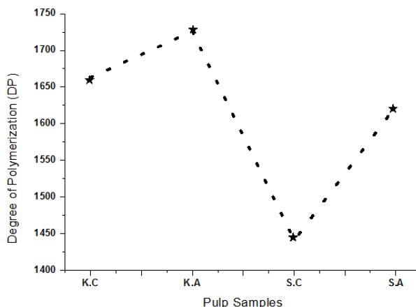
Fig. 9 Effects of acid pre-treatment on DP of unbleached pulp samples
