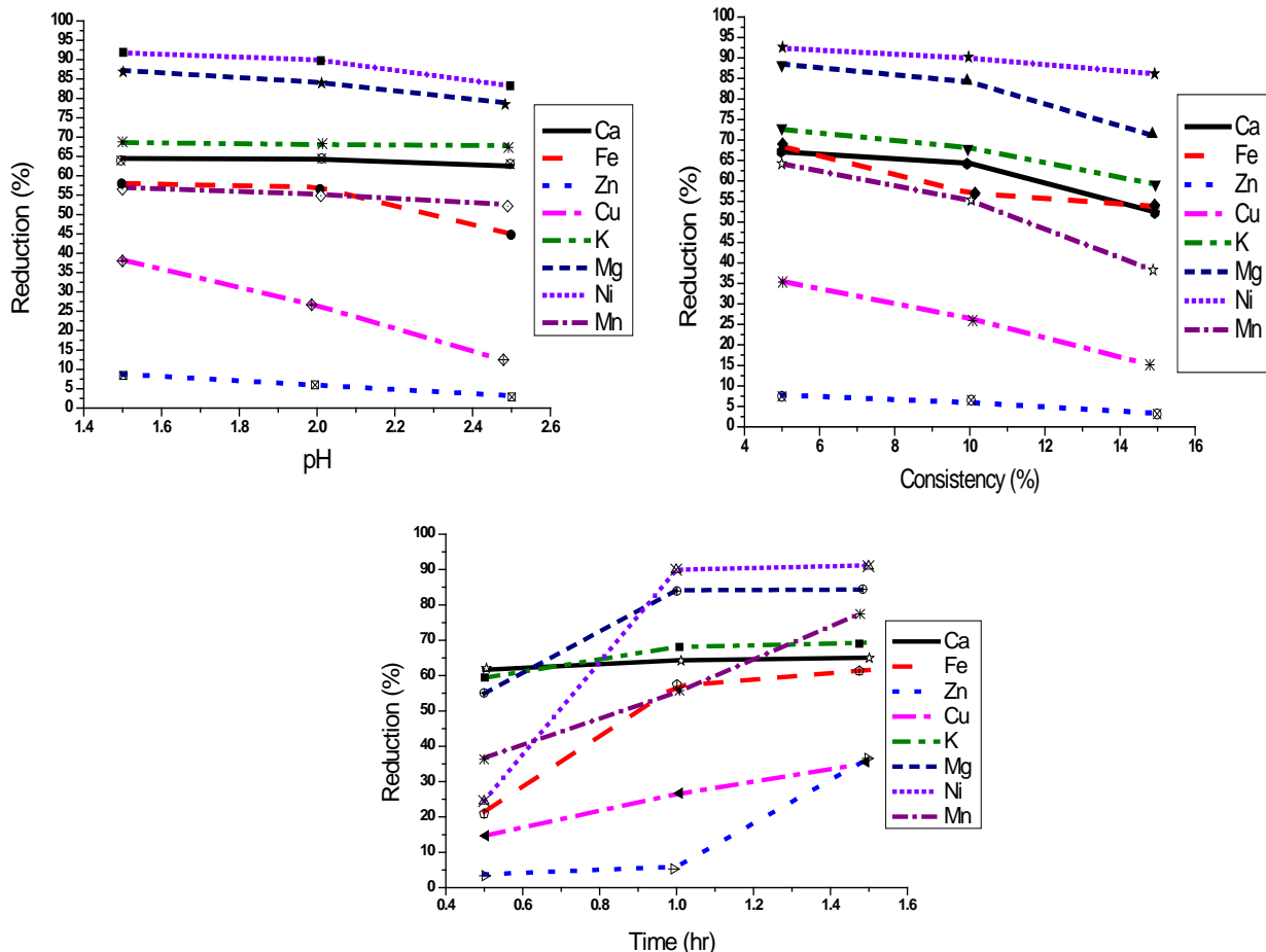
Fig. 6 Effects of pH, consistency (%) and retention time (hr) on the removal of metal ions content due to pretreatment
