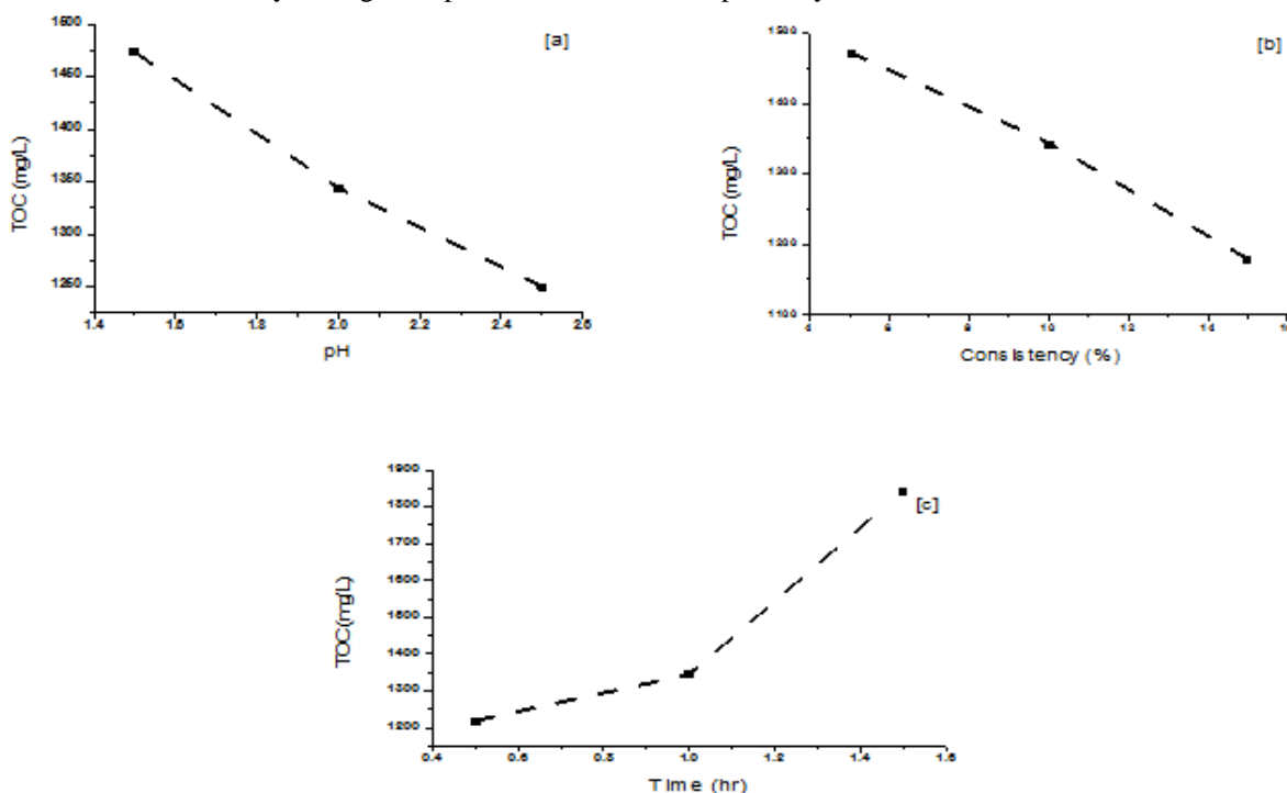
Fig. 1 Effects of [a] pH [b] consistency (%) and [c] time (hr) on total organic carbon (TOC) removal due to acid pre-treatment
