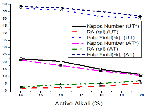
Fig. 8 Effects of acid pre-treatment on soda pulping of wheat straw (*UT- Untreated, *AT- Acid treated)
