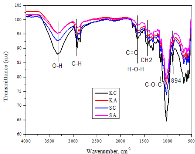
Fig. 11 FTIR spectra of kraft and soda pulp (untreated and acid treated)
