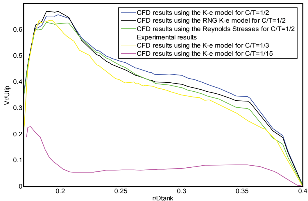
Fig. 2 Normalized radial velocity at the centerline of the impeller
