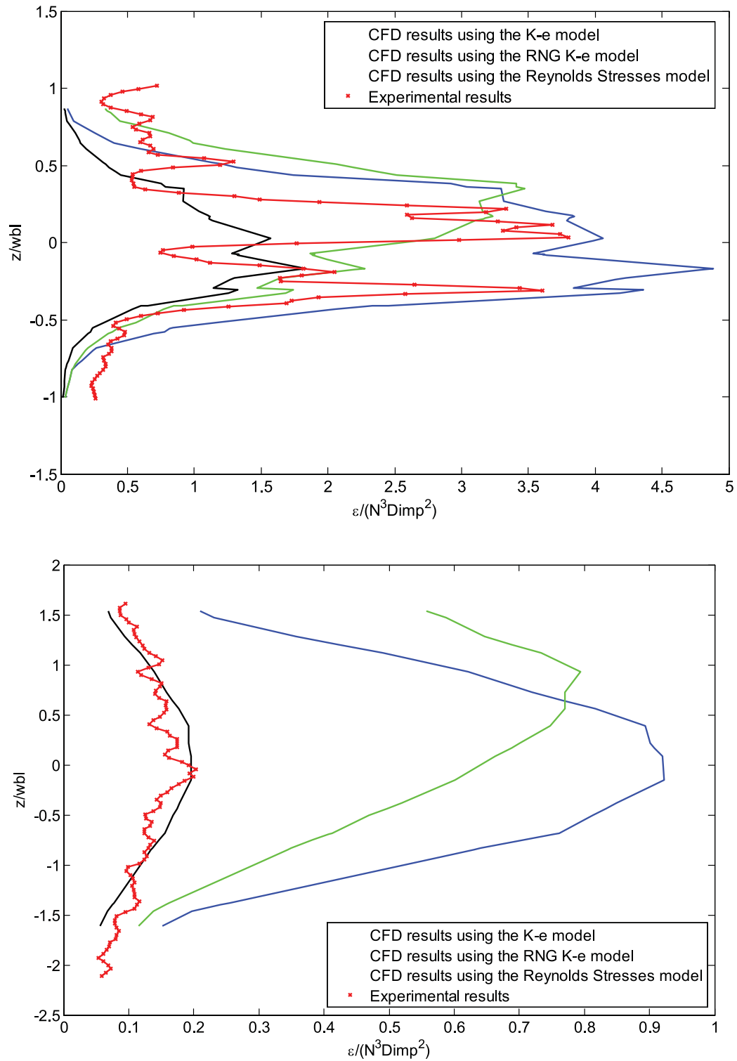
Fig. 12 Normalized Dissipation rate profiles at r/T=0.256 (top frame) and at r/T=0.315 (bottom frame) for C/D_T = 1/2 and Re=35000
