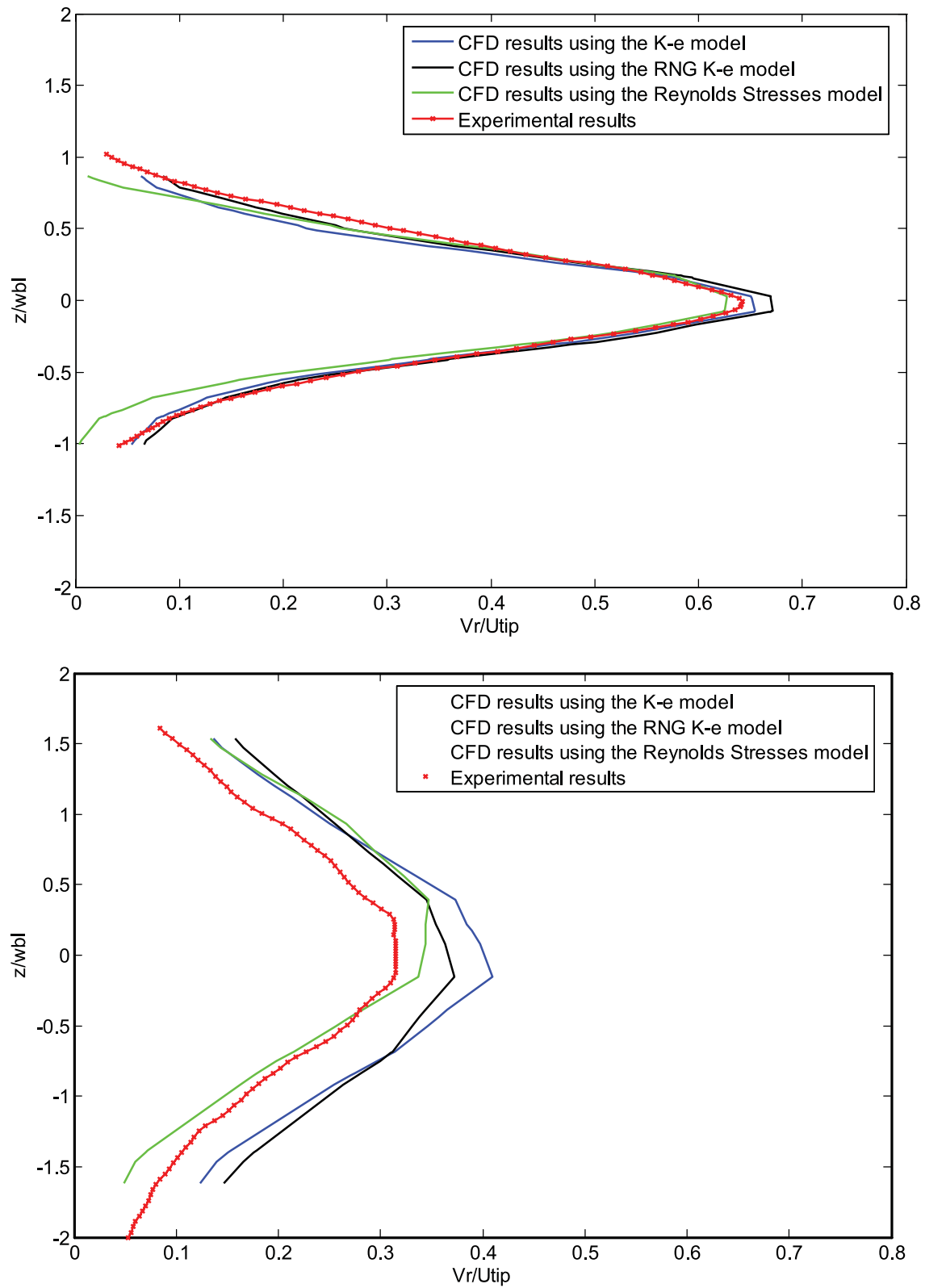
Fig.11 Normalized radial velocity profiles at r/T=0.256 (top frame) and at r/T=0.315 (bottom frame) for C/D_f = 1/2 and Re=35000
