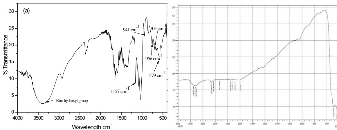
Fig.6 FT-IR Spectra of (a) \beta -CD and (b) ZnO- \beta -CD
