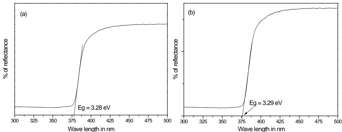
Fig.5 UV- Visible Diffused Reflectance Spectra of bare ZnO and ZnO- \beta -CD
